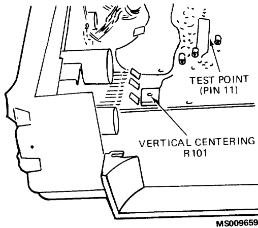
Figure 4-3. Location of Vertical Centering adjustment and test point.
