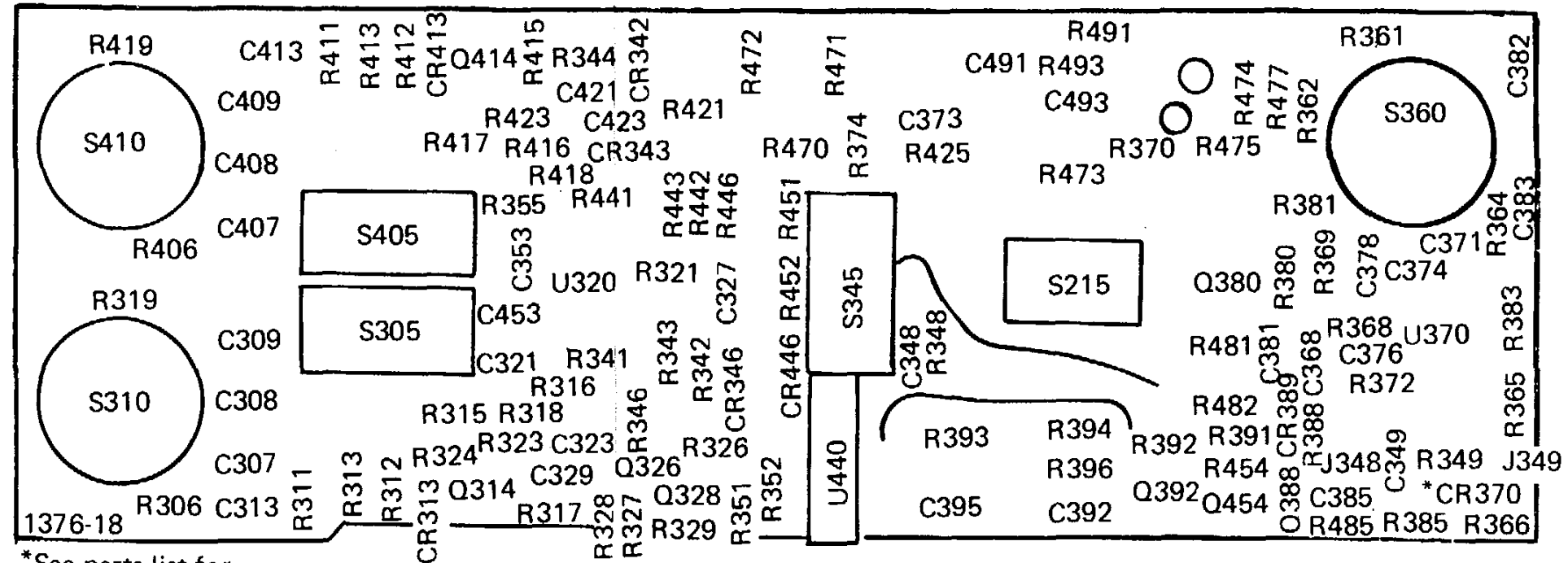
Figure 8-1A. A1 Input Circuit Board (Front).
